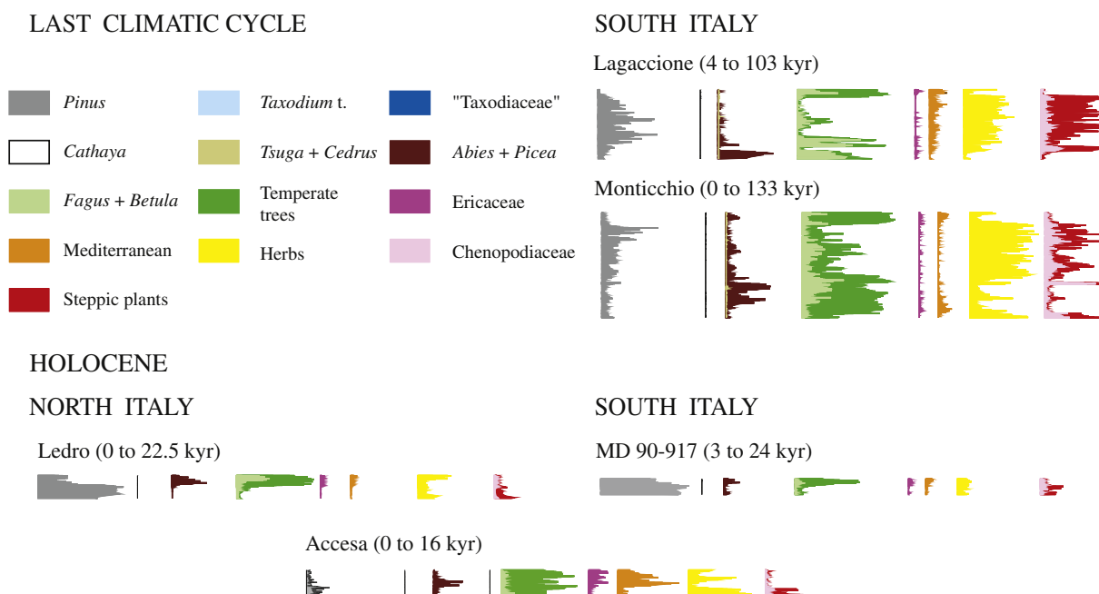
Fig. 8. Representative vegetation changes during the last climate cycle in Northern and Southern Italy.
