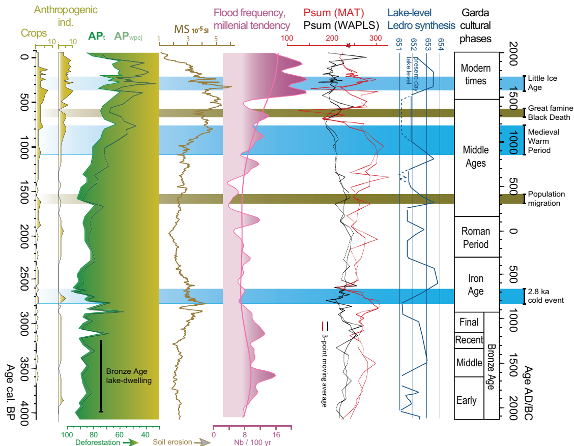
Figure 6. Ledro's record of agricultural activities, forest cover (arboreal pollen, inversed scale), erosion in the catchment (MS), flood frequency (Vannièrè et al., 2013), lake levels (Magny et al., 2012), and pollen-based reconstructed summer precipitation (the star indicates the present-day summer precipitation; Peyron et al., 2013). Climatically and non-climatically induced vegetation and land-use changes are shown in blue and brown, respectively.
